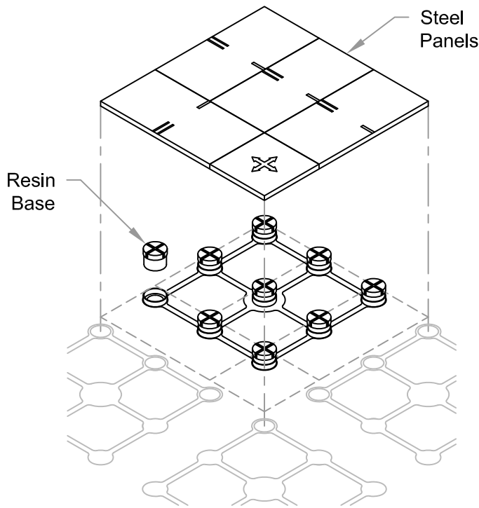
PLAN VIEW
