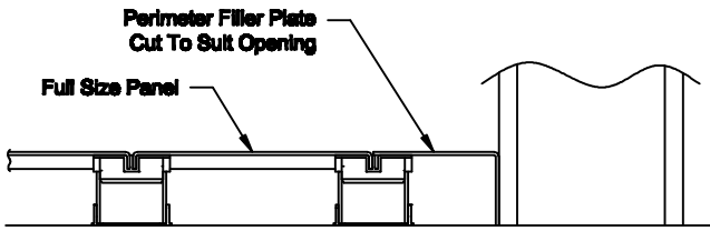
SECTION A Detail At Perimeter Filler Plate
