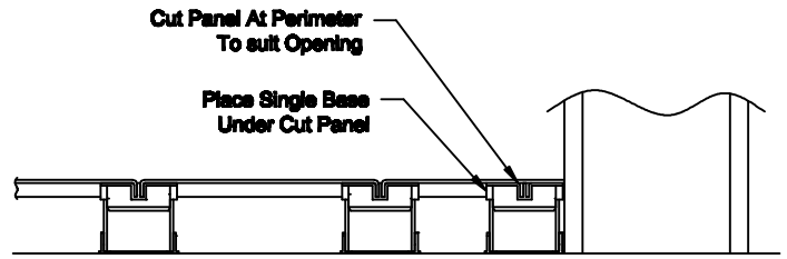
SECTION B Detail Of Cut Panel At Perimeter
