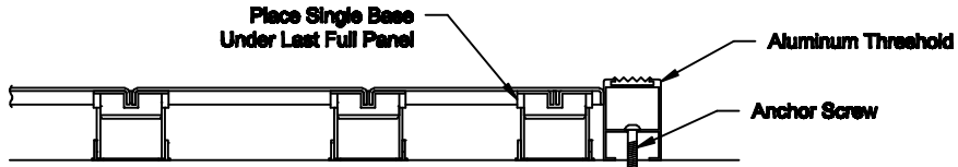
SECTION C Detail Of Threshold At Perimeter
